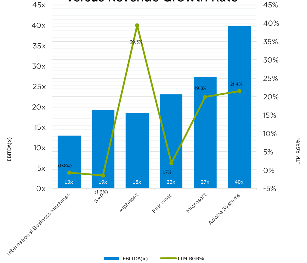
Historical Valuation Multiples versus Revenue Growth Rate
